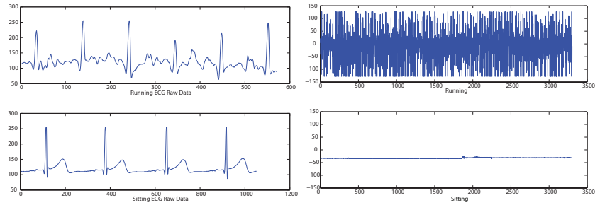
Fig. 3. (L) ECG and (R) accelerometer data from the heart-rate monitor for sitting and running.
