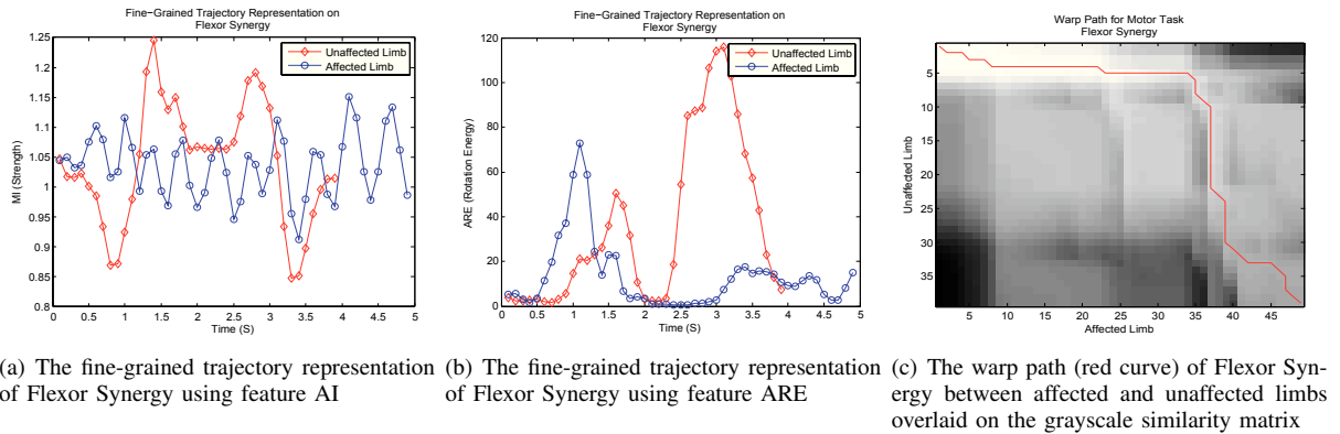
Fig. 4. The fine-grained trajectory representation and the warp path calculated from DTW of Flexor Synergy
