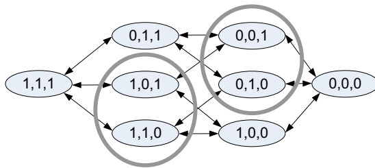
Fig. 7. Reliability model of the Follower Robot
