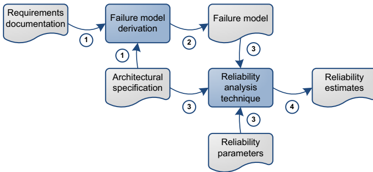
Fig. 1. Architecture-based reliability estimation process
