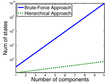
Fig. 6. Comparison of the complexity of “brute-force” and hierarchical approaches
