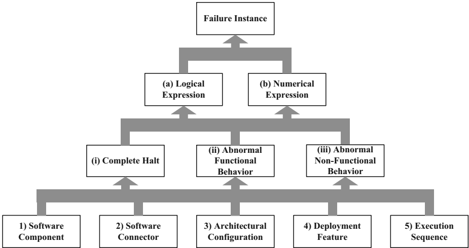
Fig. 3. Multiple dimensions in the definition of a failure instance
