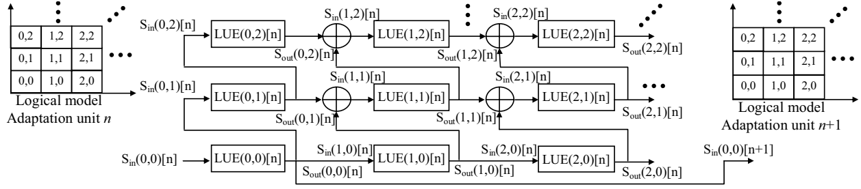
Fig. 3 Multi-dimensional state propagating encryption for generalized scalable bit-streams. A 2-dim example is shown. LUE( i,j )[ n ] is the Logical Unit Encrypter for the ( i,j )th logical unit of adaptation unit n . It is implicit here that each LUE takes in a logical unit plaintext having a specified length and yields the corresponding ciphertext based on a key.
