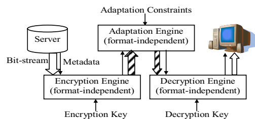
Fig. 1 Format-independent delivery architecture.
