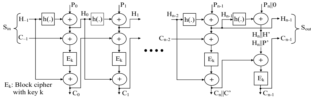
Fig. 4 LUE based on Accumulated Block Chaining (ABC) mode. When h(X)=0 , ABC becomes Infinite Garble Extension (IGE) mode.
