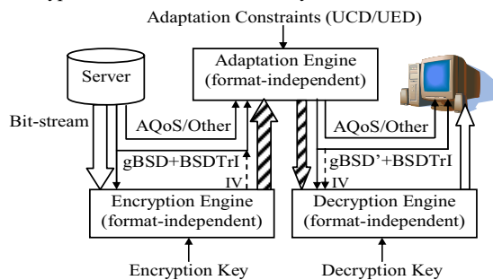
Fig. 5 Format-Independent Encryption-Adaptation-Decryption chain based on MPEG-21 DIA descriptions. Initialization vectors (IV) that need to be sent to the decryption engine can be integrated into the gBSD during encryption.
