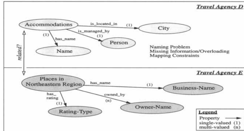
Fig. 3. Example 1. Semantic heterogeneity in FOTA.
