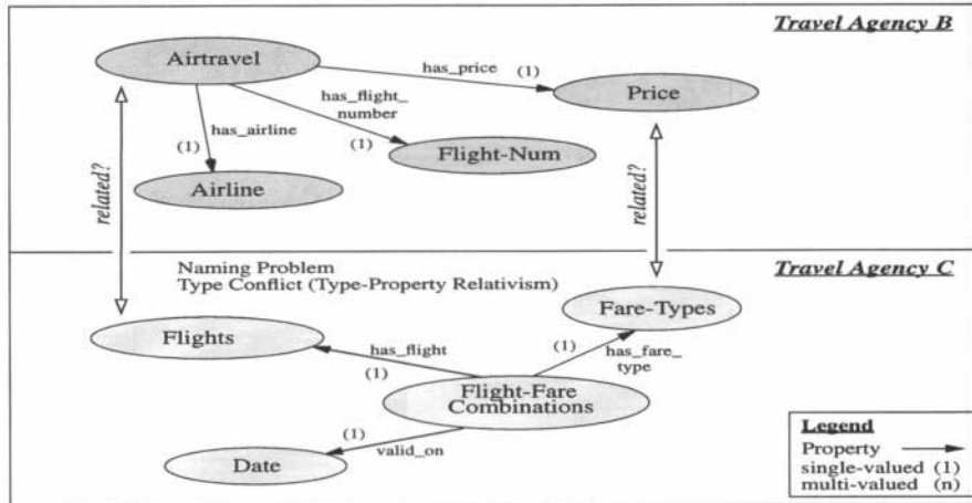
Fig. 4. Example 2. Semantic heterogeneity in FOTA.
