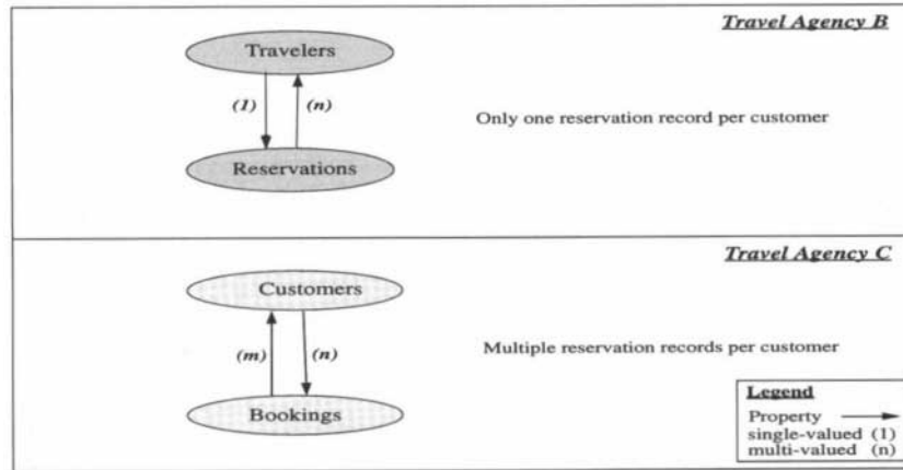
Fig. 5. Example 3. Semantic heterogeneity in FOTA.
