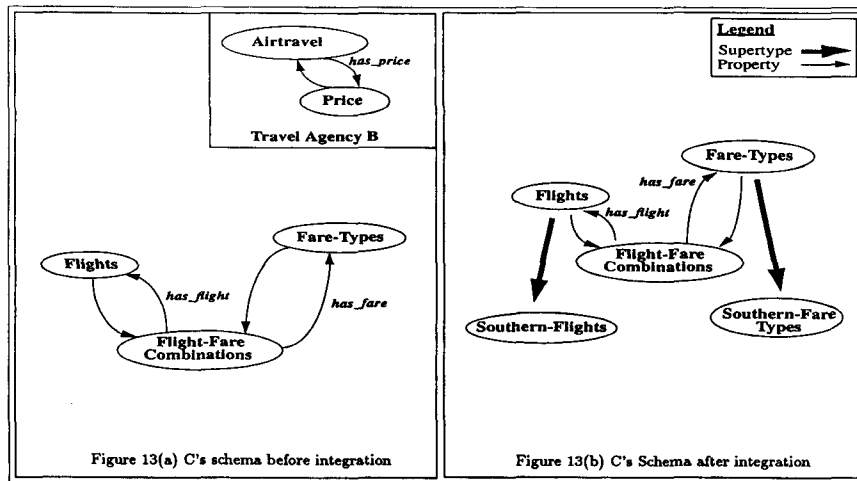
Fig. 13. Example 2. Integration of several inter-related objects.
