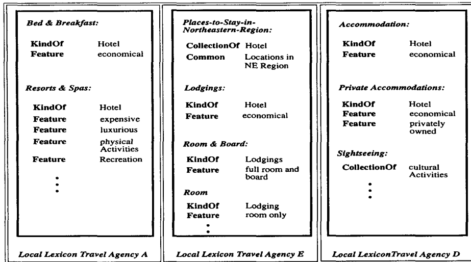
Fig. 9. A partial view of three local lexica.
