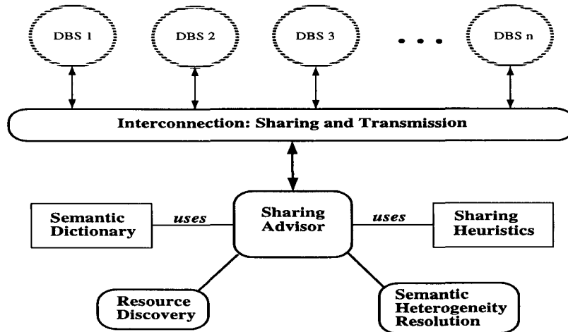
Fig. 6. Interoperability in a federation of databases.
