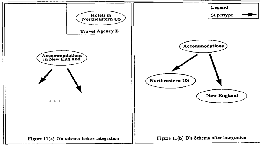
Fig. 11. Integration of two related objects.
