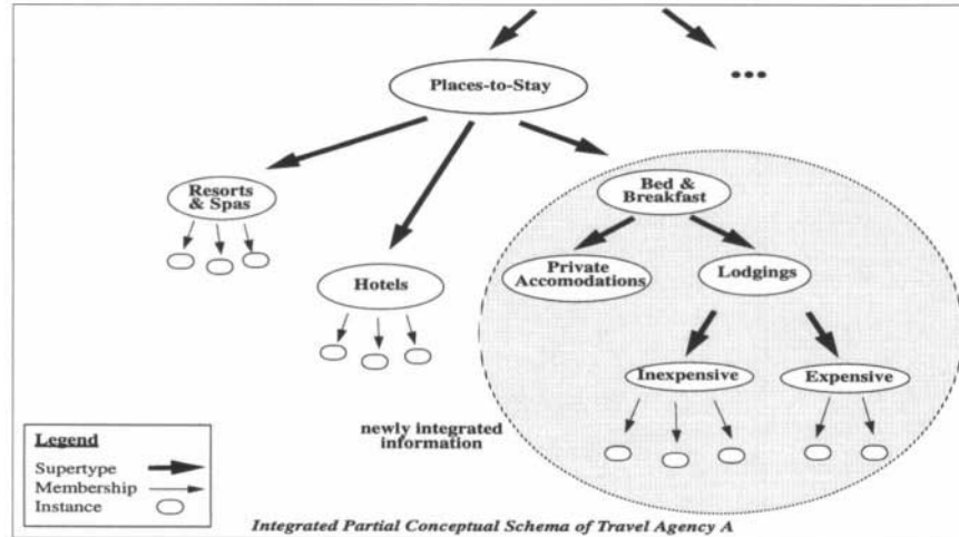
Fig. 8. Travel agency A 's schema after the importation of "Bed & Breakfast"-like information.
