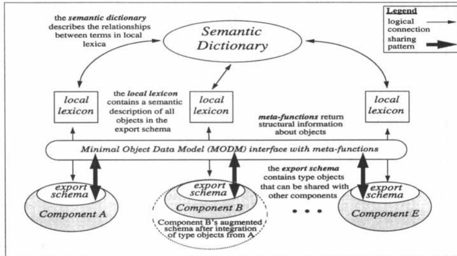
Fig. 10. Sharing architecture and the various interactions among its components.
