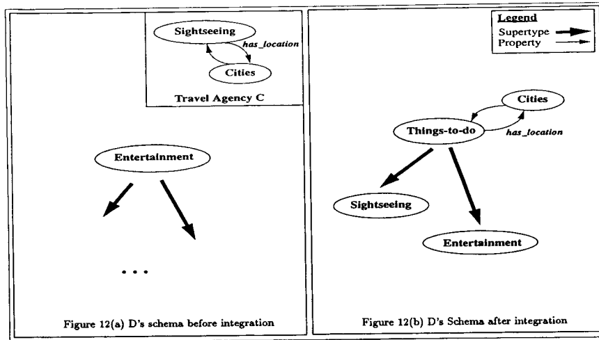
Fig. 12. Example 1. Integration of several inter-related objects.
