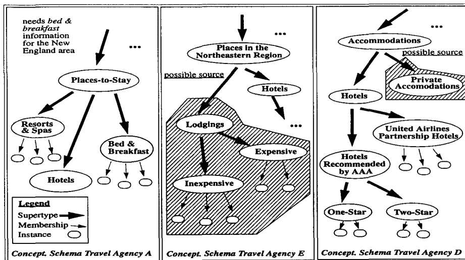
Fig. 7. Three partial conceptual schemas for travel agencies A , E , and D .
