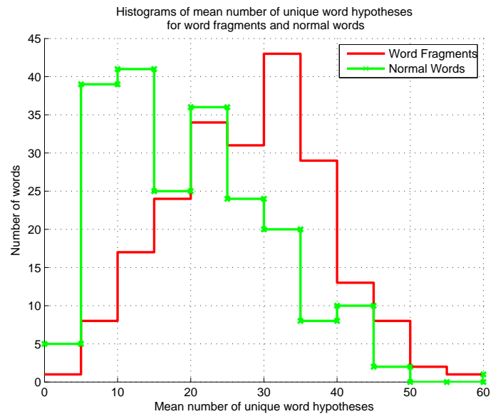
Fig. 2. Histograms of the mean number of unique word hypotheses across the ASR output lattice during word fragments and normal words. 211 samples each of word fragments and normal words were taken from the San Diego corpus [3].
